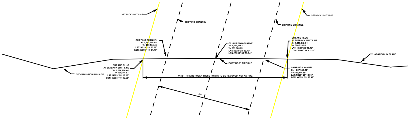
PLAN VIEW NOT TO SCALE
